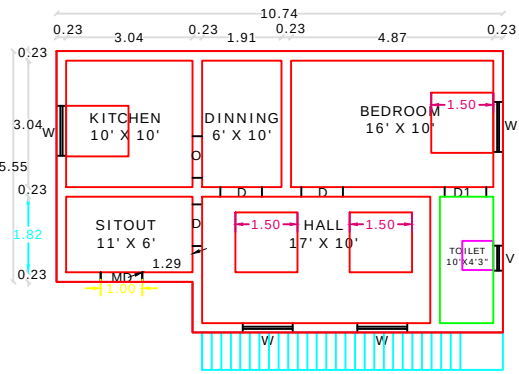
GROUND FLOOR RESIDENTIAL PLAN
