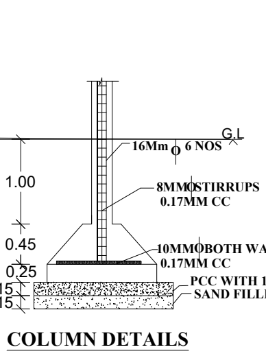
COLUMN DETAILS
