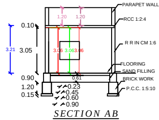
SECTION AB
