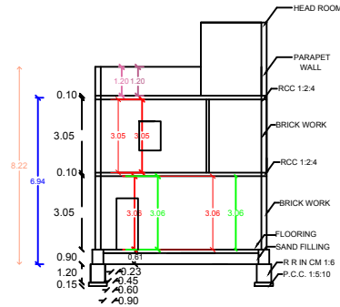
SECTION AB
