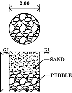
RAINWATER HARVESTING
