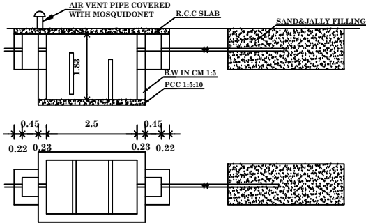
PLAN&SECTION OF SEPTIC TANK TRENCH
