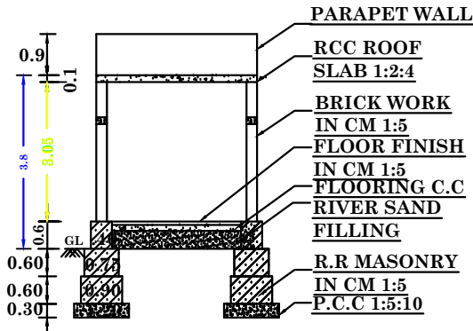
SECTION ON AA1
