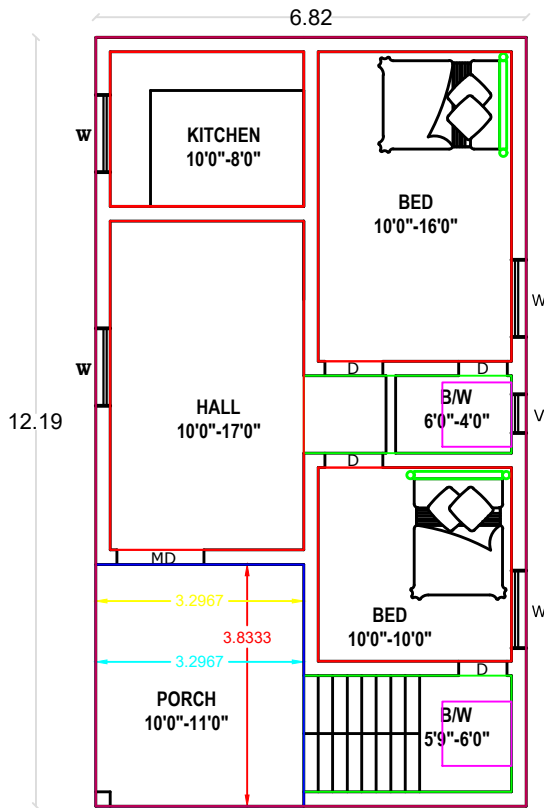
PLAN
