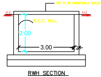
RWH SECTION
