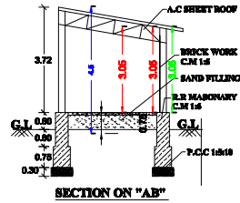
SECTION ON "AB"
