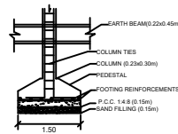
FOUNDATION DETAILS
