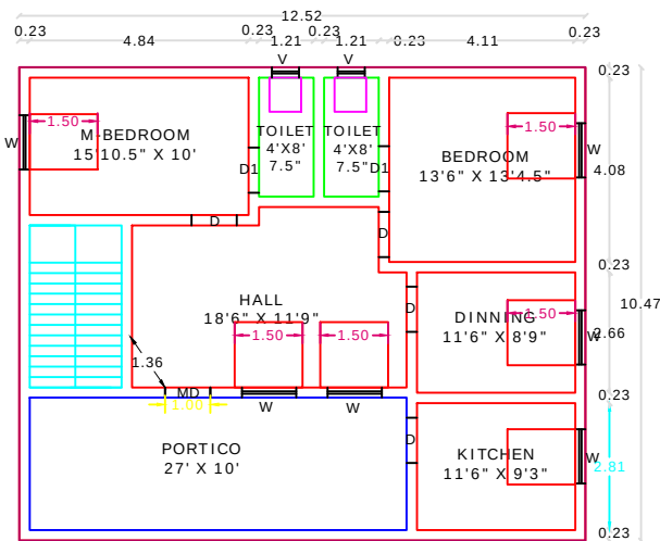
GROUND FLOOR RESIDENTIAL PLAN
