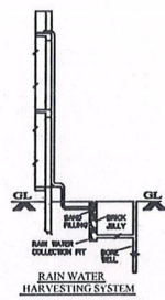
RAIN WATER HARVESTING SYSTEM
