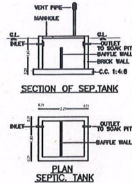
PLAN SEPTIC TANK
