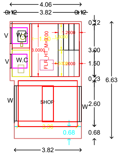
G.FLOOR PLAN
