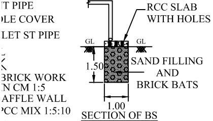
SECTION OF BS
