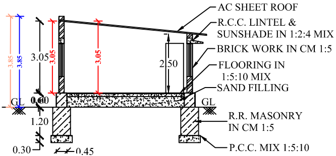
SECTION OF "AB"
