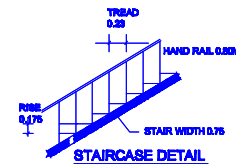
STAIRCASE DETAIL
