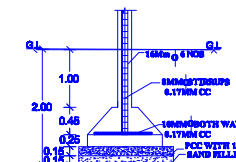
COLUMN DETAILS
