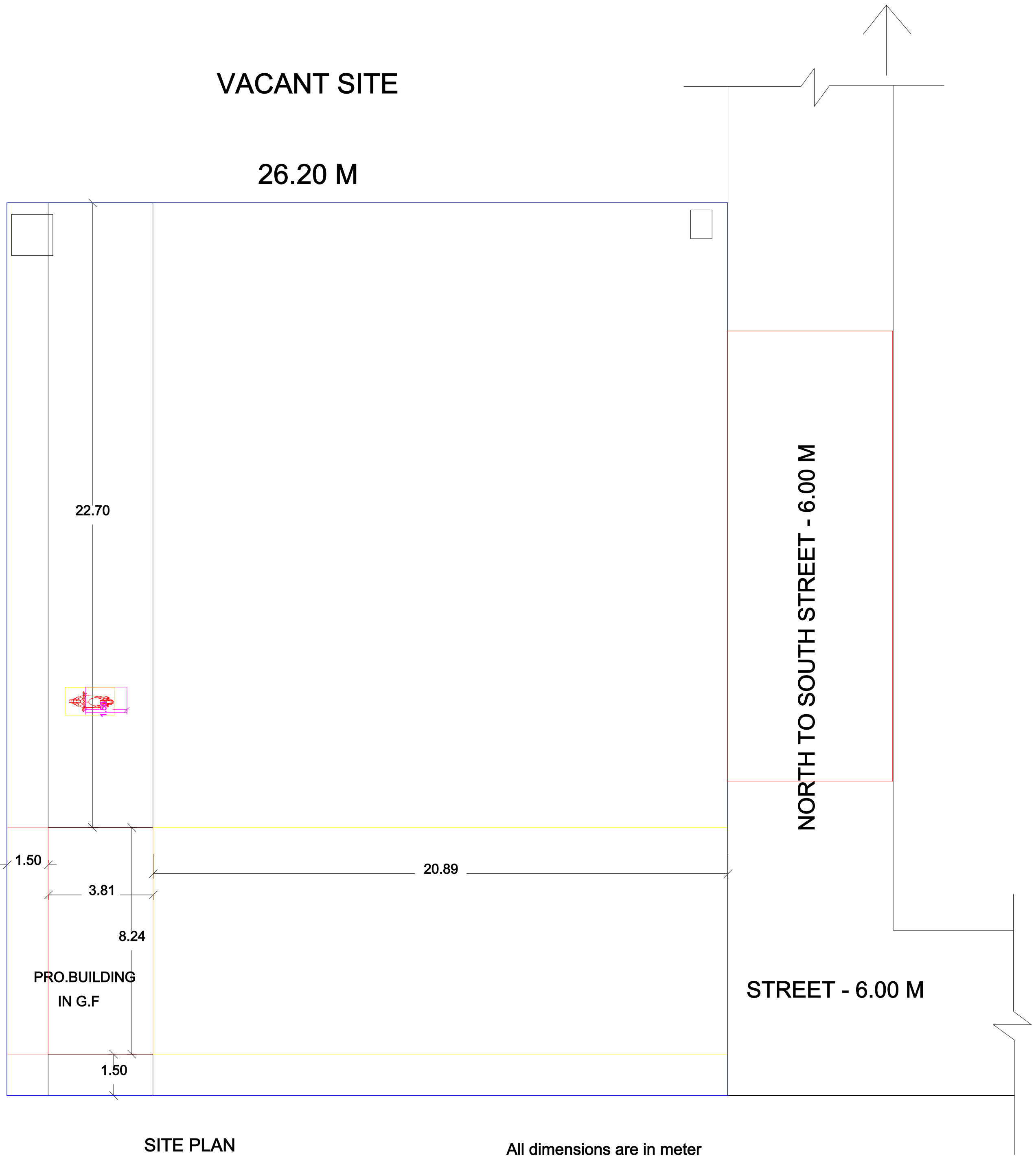
SITE PLAN
