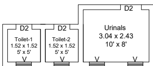
PRO. TOILET & URINAL PLAN
