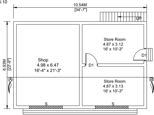
PRO. GROUND FLOOR
