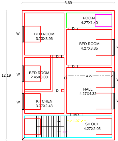
PROPOSED GF PLAN
