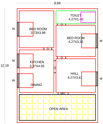
PROPOSED FF PLAN
