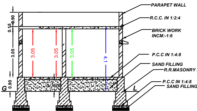
SECTION "AB"
