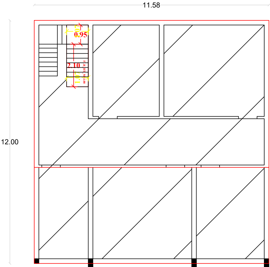
EXG.FIRST FLOOR PLAN
