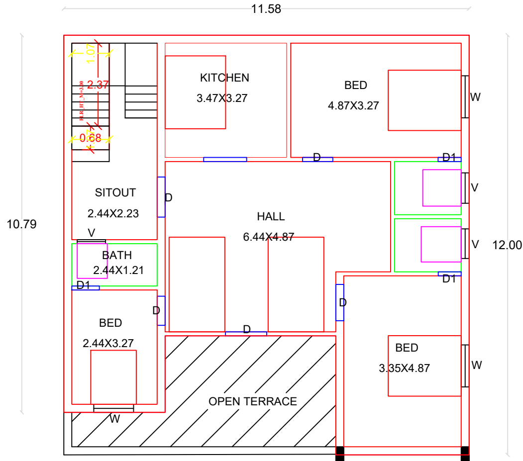
PRO.SECOND.FLOOR PLAN
