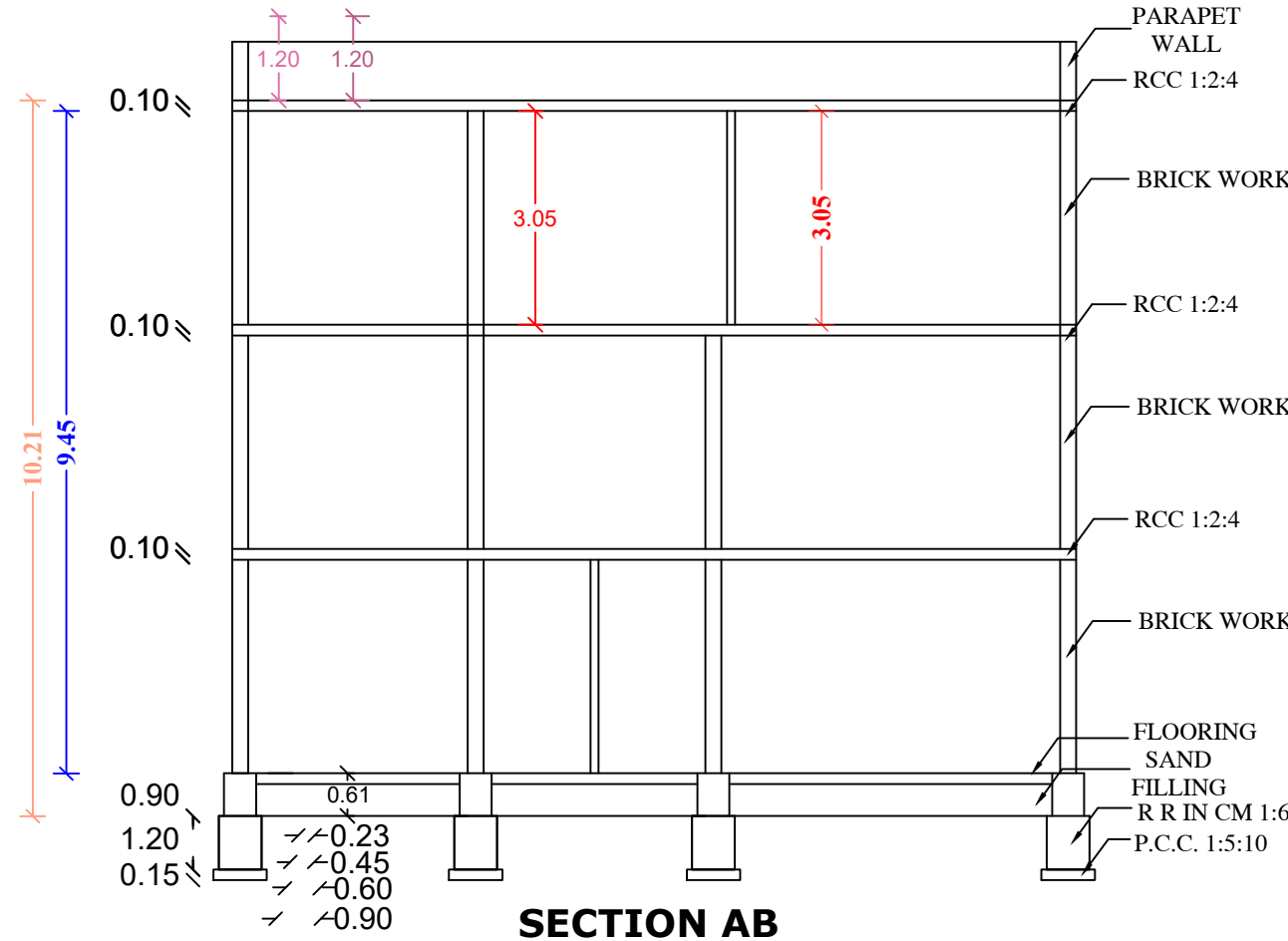
SECTION AB
