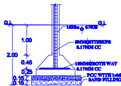
COLUMN DETAILS
