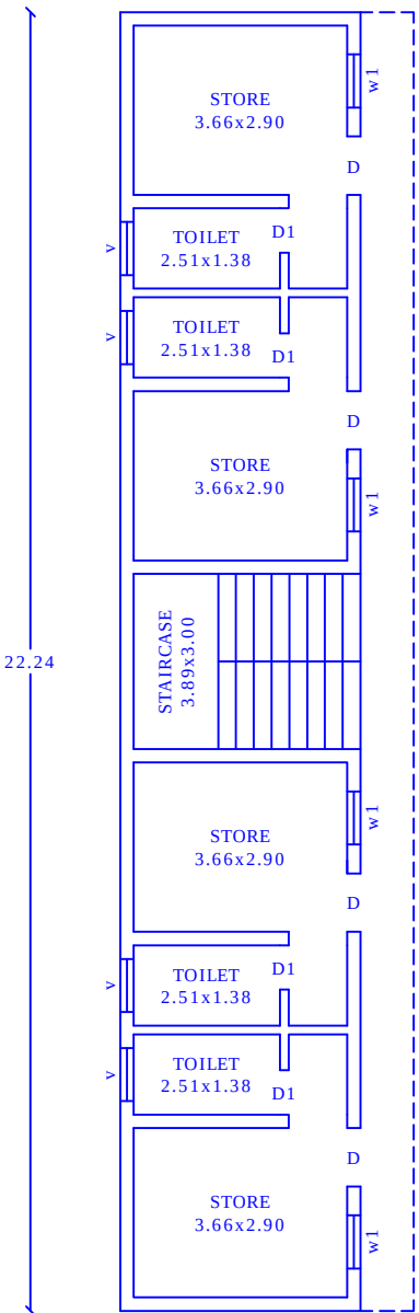
PRO FIRST FLOOR PLAN
