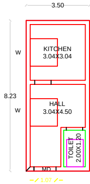
PROPOSED GF PLAN
