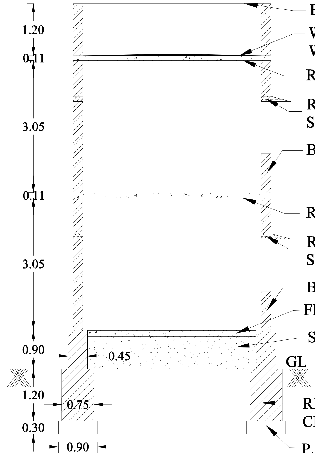
SECTION OF "AB"
