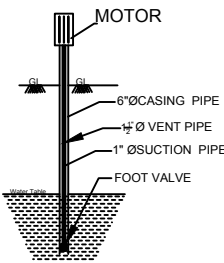
SEC. OF BOREWELL
