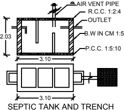
SEPTIC TANK AND TRENCH
