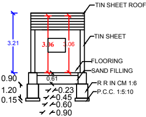
SECTION AB
