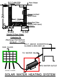
SOLAR WATER HEATING SYSTEM
