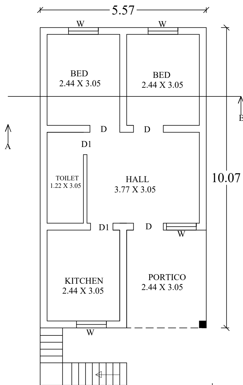
PLAN
