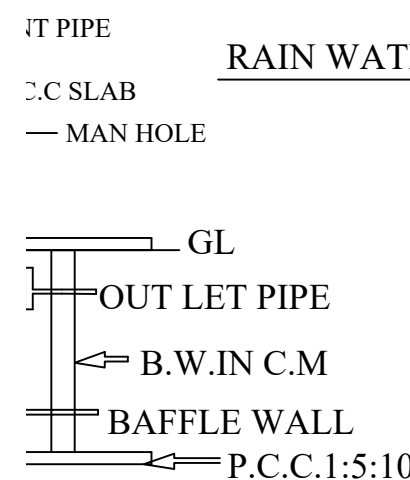
SECTION ON SEPTIC TANK
