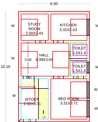
PROPOSED GF PLAN
