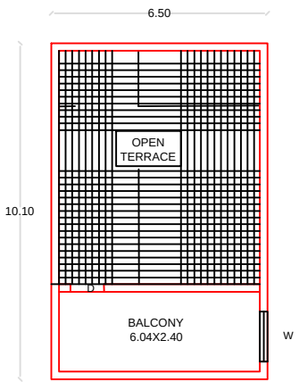
PROPOSED FF PLAN
