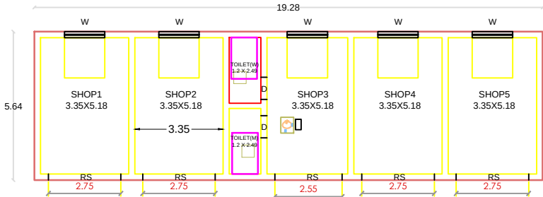
PRO SHOP PLAN
