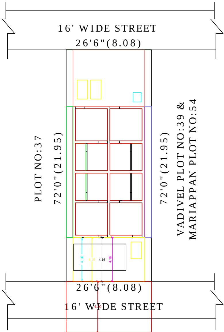
SITE PLAN
