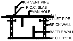
SECTION ON SEPT.TANK
