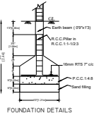
FOUNDATION DETAILS
