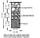
SECTION OF RAIN WATER COLLECTION PIT DETAILS
