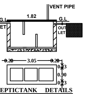
SEPTICTANK DETAILS
