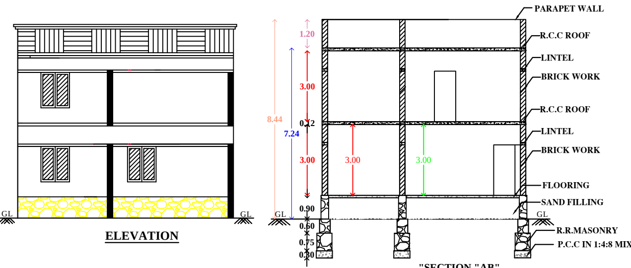
"SECTION "AB"
