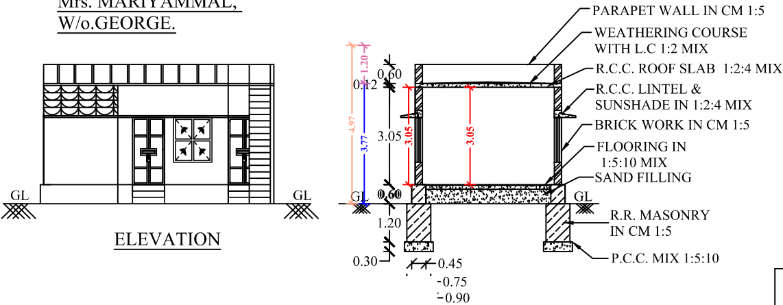
SECTION OF "AB"
