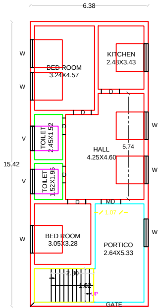
PROPOSED GF PLAN
