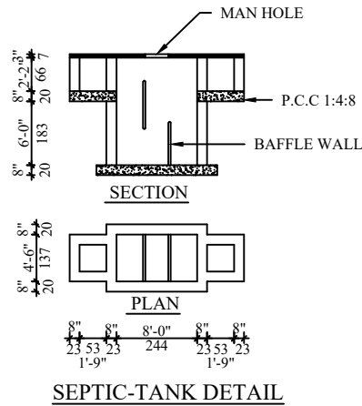
SEPTIC-TANK DETAIL
