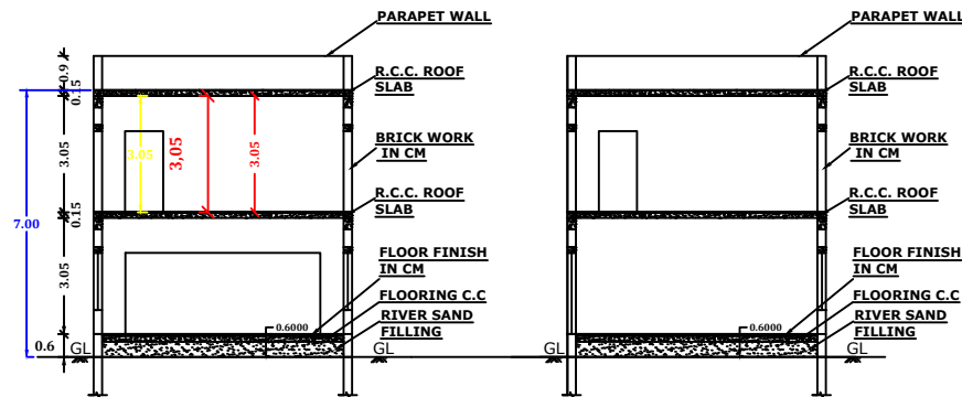
SECTION ON AA1
