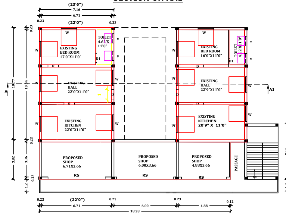
PROPOSED/EXISTING FIRST FLOOR PLAN
