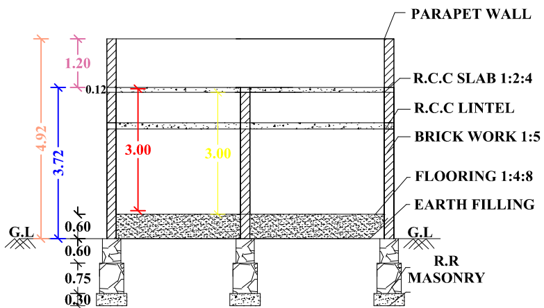
"SECTION "AB"
