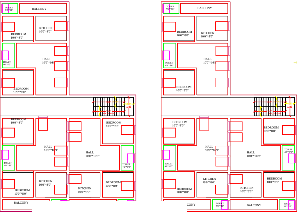
PROPOSED F.FLOOR PLAN
