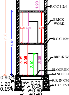
SECTION AB
