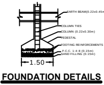
FOUNDATION DETAILS
