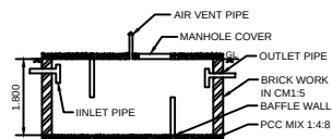
SECTION OF SEPTIC TANK
