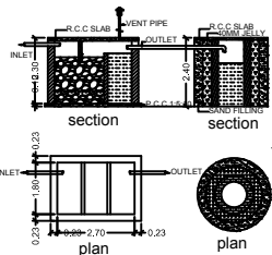
1000 GALLONS CAPACITY SEPTIC TANK (NTS)
