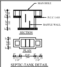
SEPTIC-TANK DETAIL
