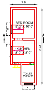
ROUND FLOOR PLAN
