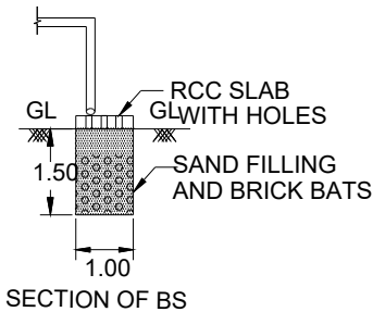
SECTION OF BS
