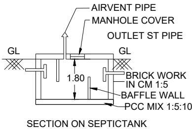
SECTION ON SEPTICTANK
