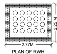
PLAN OF RWH
