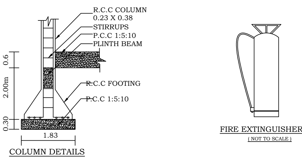
COLUMN DETAILS
