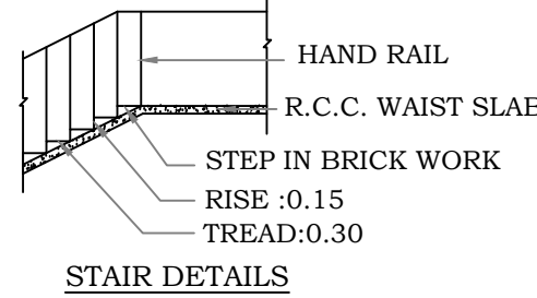
STAIR DETAILS
