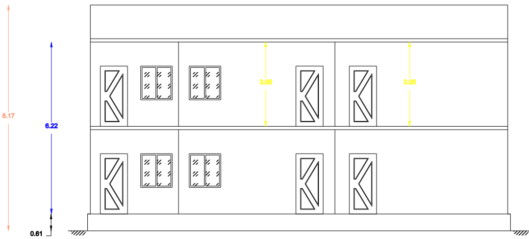
FRONT ELEVATION
