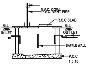
SEC. OF SEPTIC TANK
