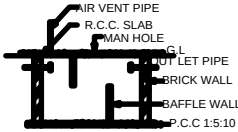
SECTION ON SEPTIC TANK
