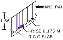
STAIRCASE
