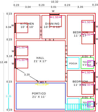
GROUND FLOOR RESIDENTIAL PLAN
