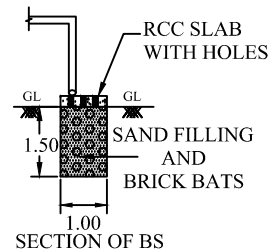
SECTION OF BS
