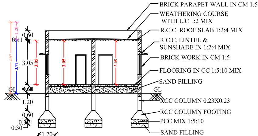
SECTION OF "AB"
