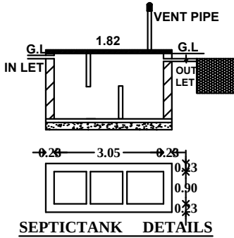
SEPTICTANK DETAILS
