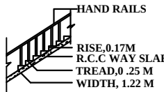
SECTION ON STAIR
