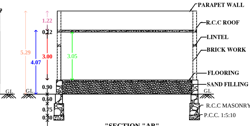
"SECTION "AB"
