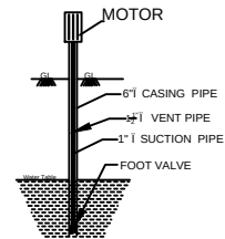
SEC. OF BOREWELL
