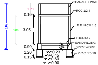
SECTION AB
