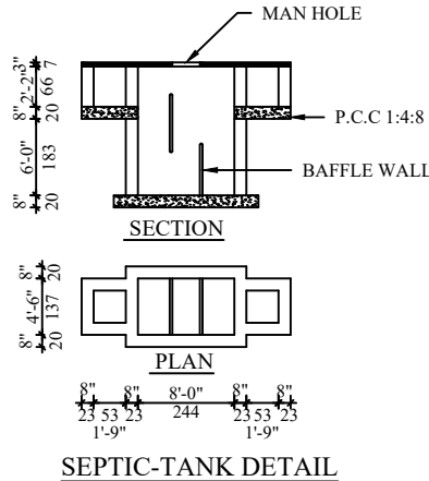
SEPTIC-TANK DETAIL
